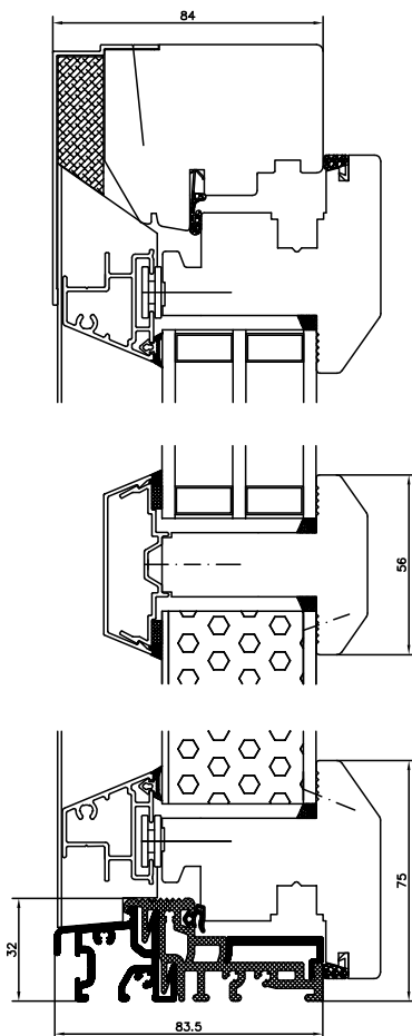
Threshold+spacer+upper frame
