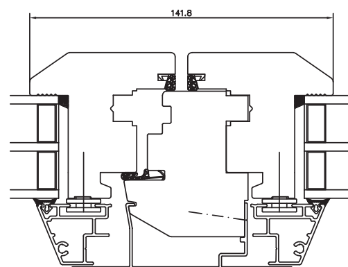
Central roller sash
