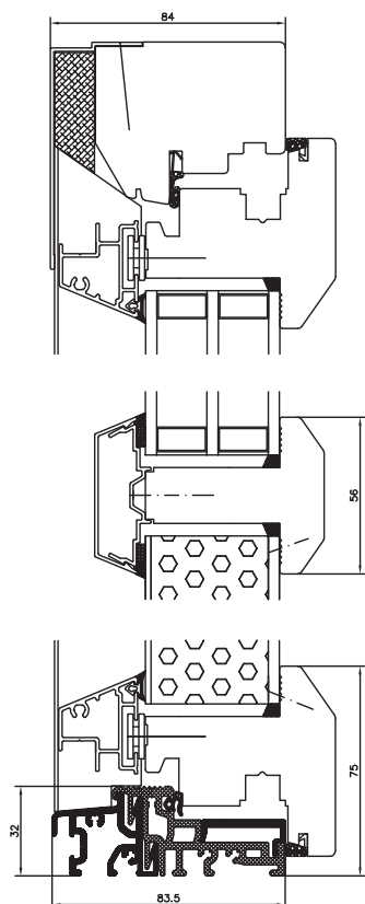
Threshold + spacer + upper frame
