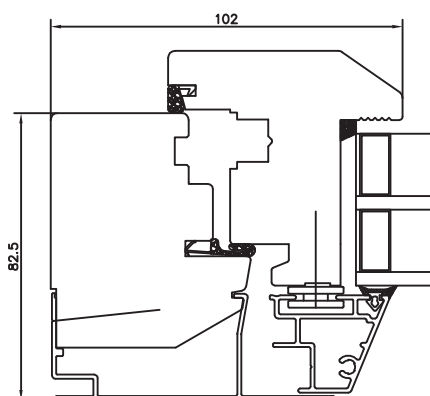
Side frame
