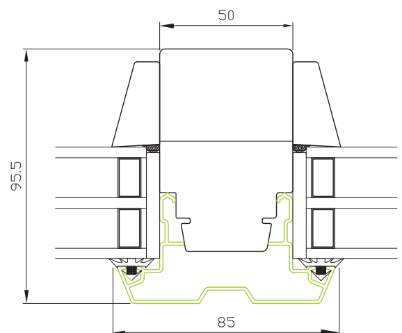
Vertical/horizontal impost
