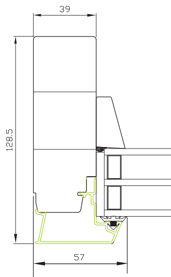
Side frame
