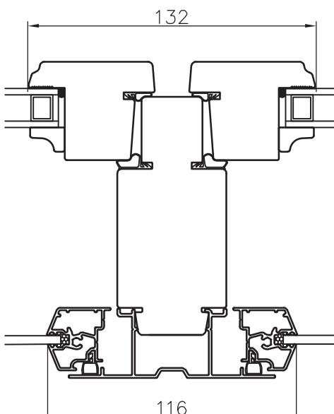
Vertical impost
