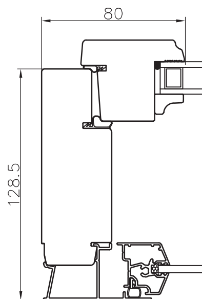
Side frame
