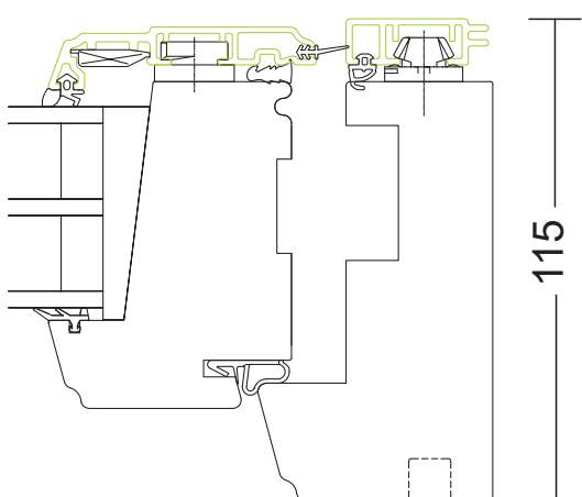
Side frame
